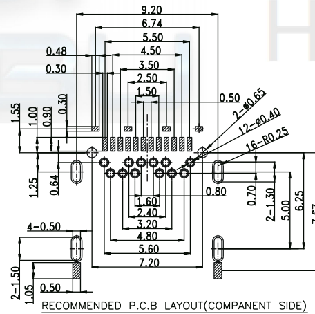
RECOMMENDED P.C.B LAYOUT (COMPONENT SIDE) PCB THICKNESS: 2.0±0.05mm
