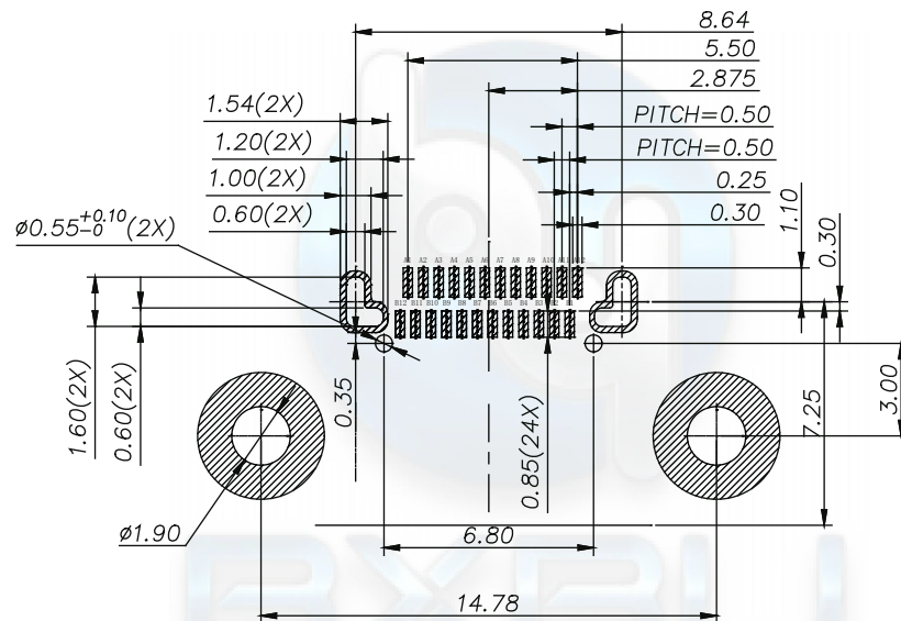
RECOMMENDED PCB LAYOUT(TOP VIEW) THICKNESS 0.60MM;DEFAULT TOLERANCE: ±0.05
