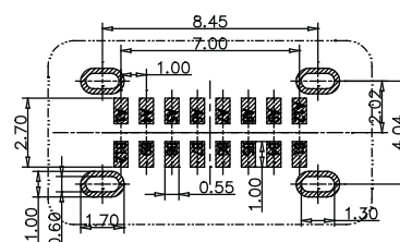
RECOMMEND P.C.B LAYOUT TOLERANCE UNSPECIFIED ±0.05mm
