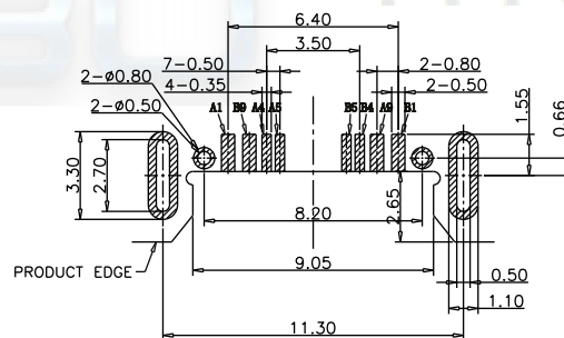
RECOMMEND P.C.B LAYOUT (COMPONENT SIDE) TOLERANCE FOR PCB LAYOUT IS ±0.05
