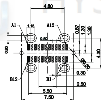
RECOMMENDED P.C.B. LAYOUT TOLERANCE UNSPECIFIED \pm 0.05\text{mm}
