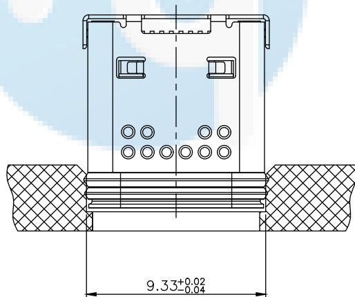
SECTION X-X
