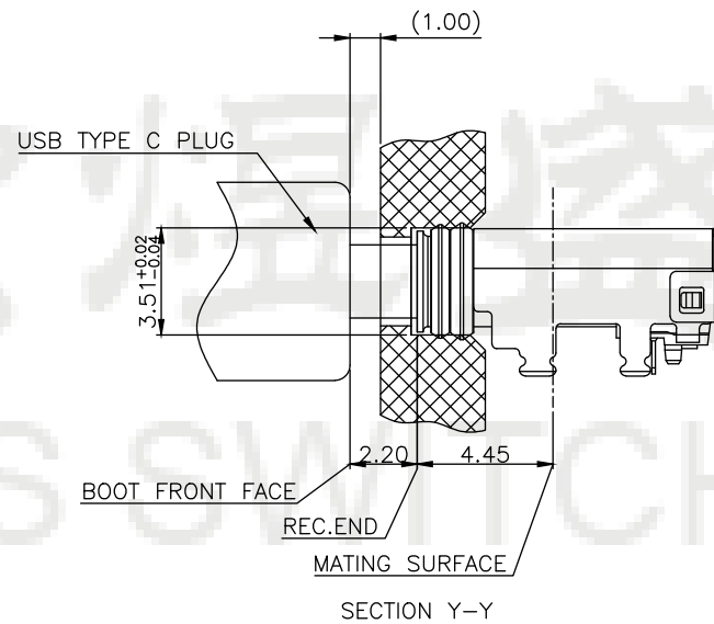
SECTION Y-Y
