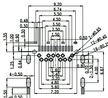
RECOMMENDED P.C.B LAYOUT (COMPONENT SIDE) PCB THICKNESS: 2.0±0.05mm
