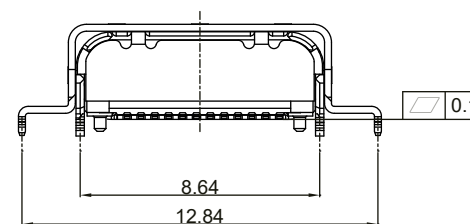
MOUNTING CONDITION(REF.)
