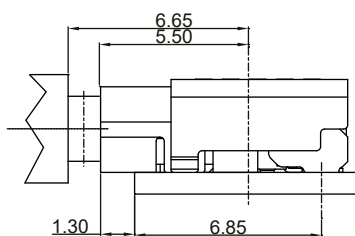
MATED CONDITION(REF.)
