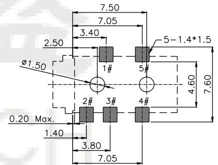
RECOMMENDED P.C.B LAYOUT TOP VIEW (TOLRANCE:±0.05)
