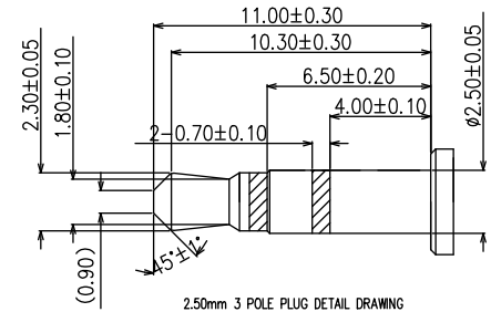
2.50mm 3 POLE PLUG DETAIL DRAWING
