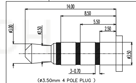
(Φ3.50mm 4 POLE PLUG)
