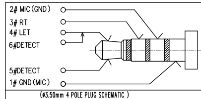
(Φ3.50mm 4 POLE PLUG SCHEMATIC)
