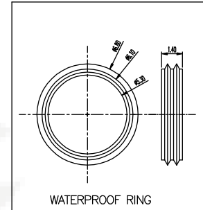
WATERPROOF RING
