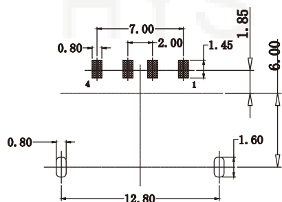
RECOMMENDED PCB LAYOUT THICKNESS=1.0mm (TOLERANCES ±0.05)
