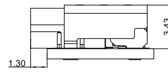
MOUNTING CONDITION(REF.)
