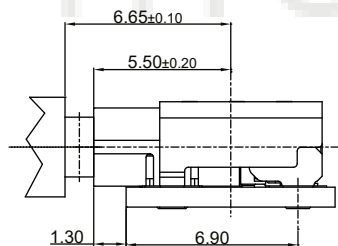
MATED CONDITION(REF.)
